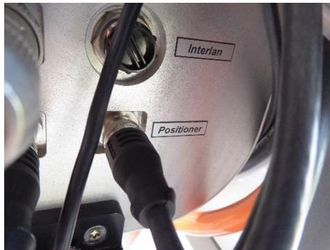
Connected positioner cable.
