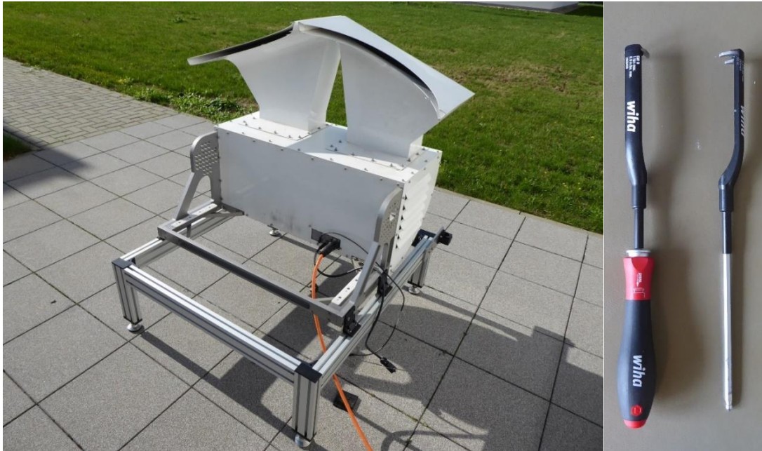
Left: The blower with air baffles and connected cables. Right: Tool to tighten the connectors.
