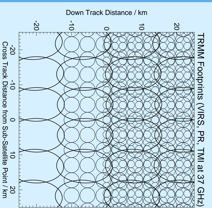
Figure 1: Scan pattern of the three main TRMM instruments in the center of the satellite track.
