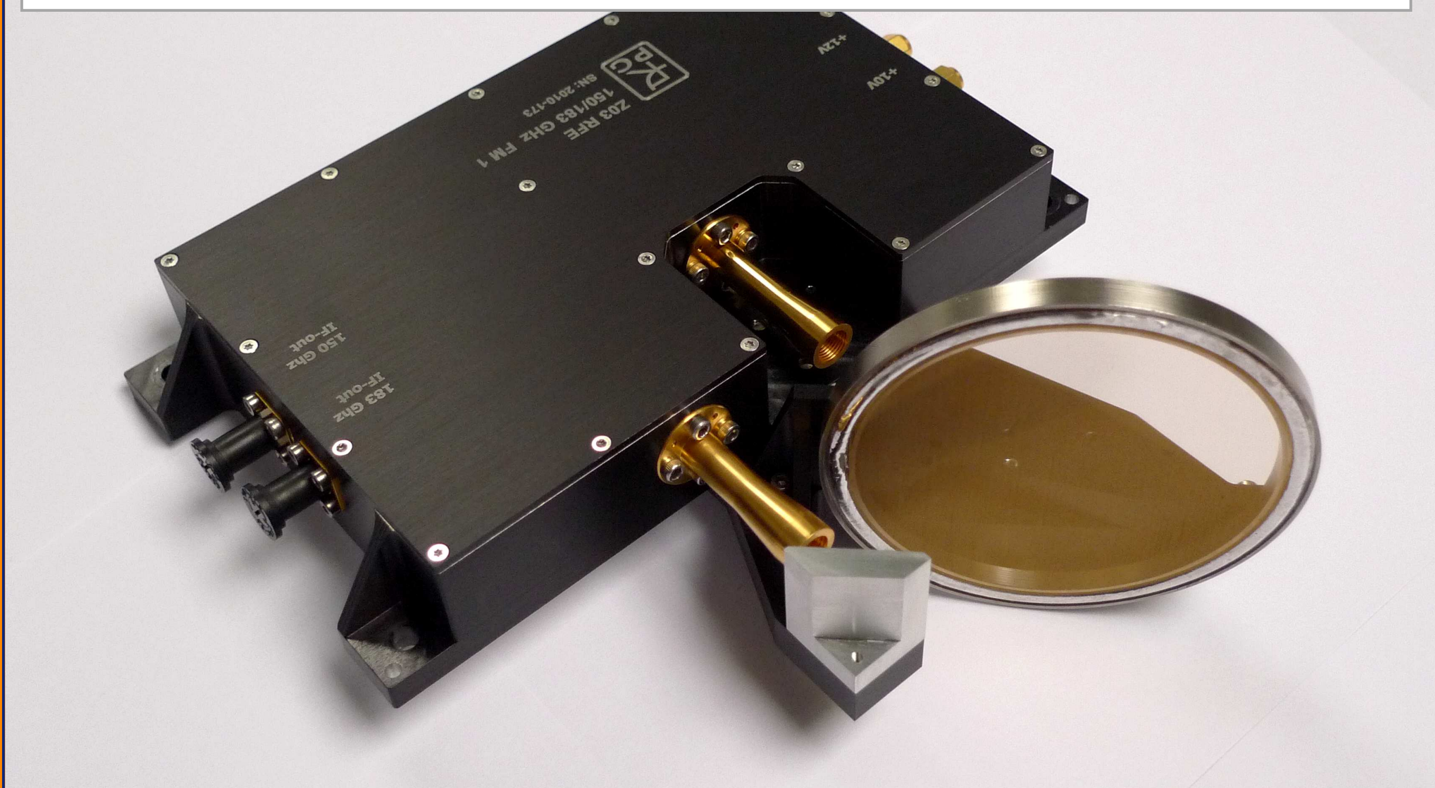
150/183 GHz Dual, China, FY-3
