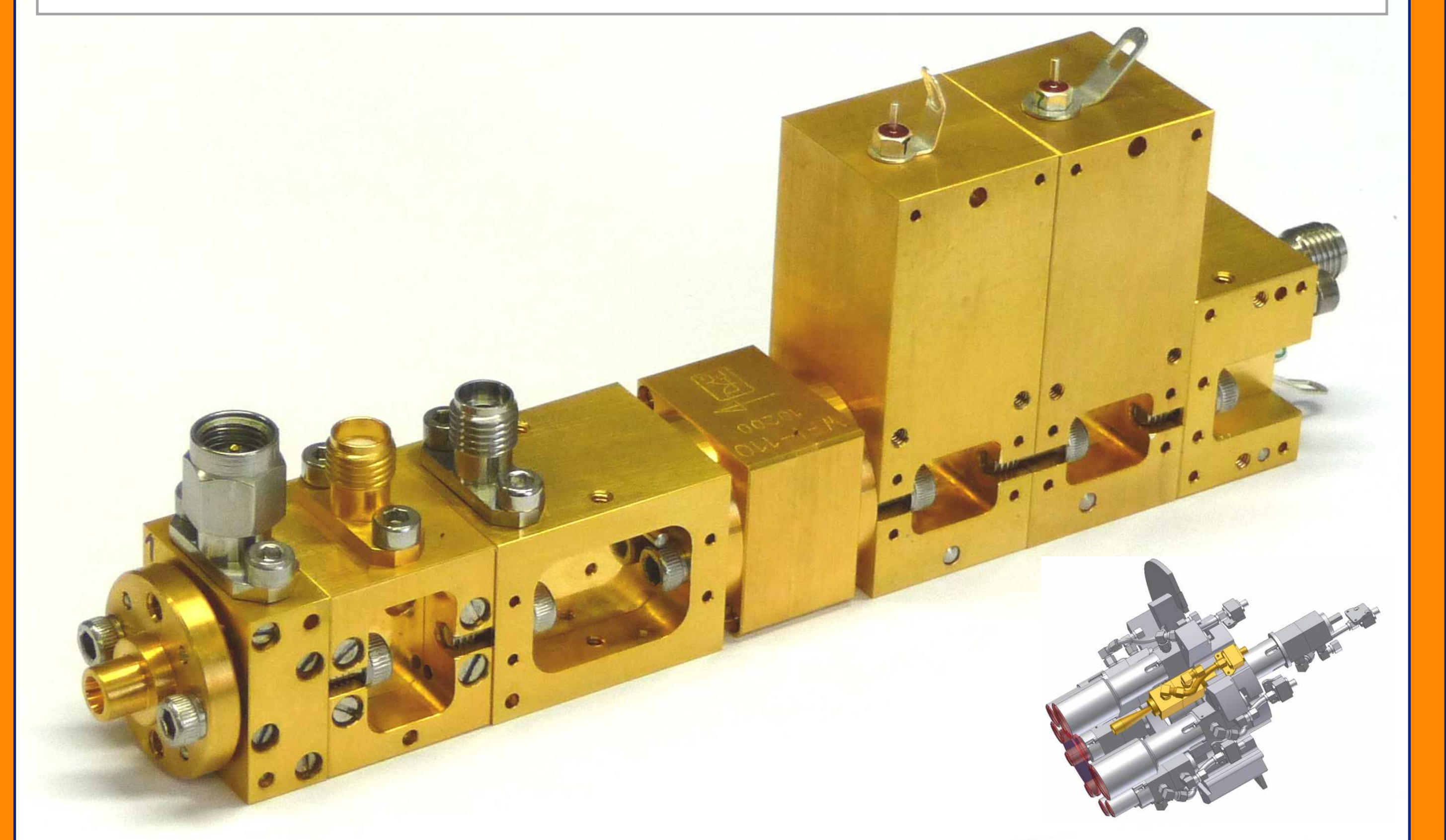
664 GHz Airborne Demonstrator
