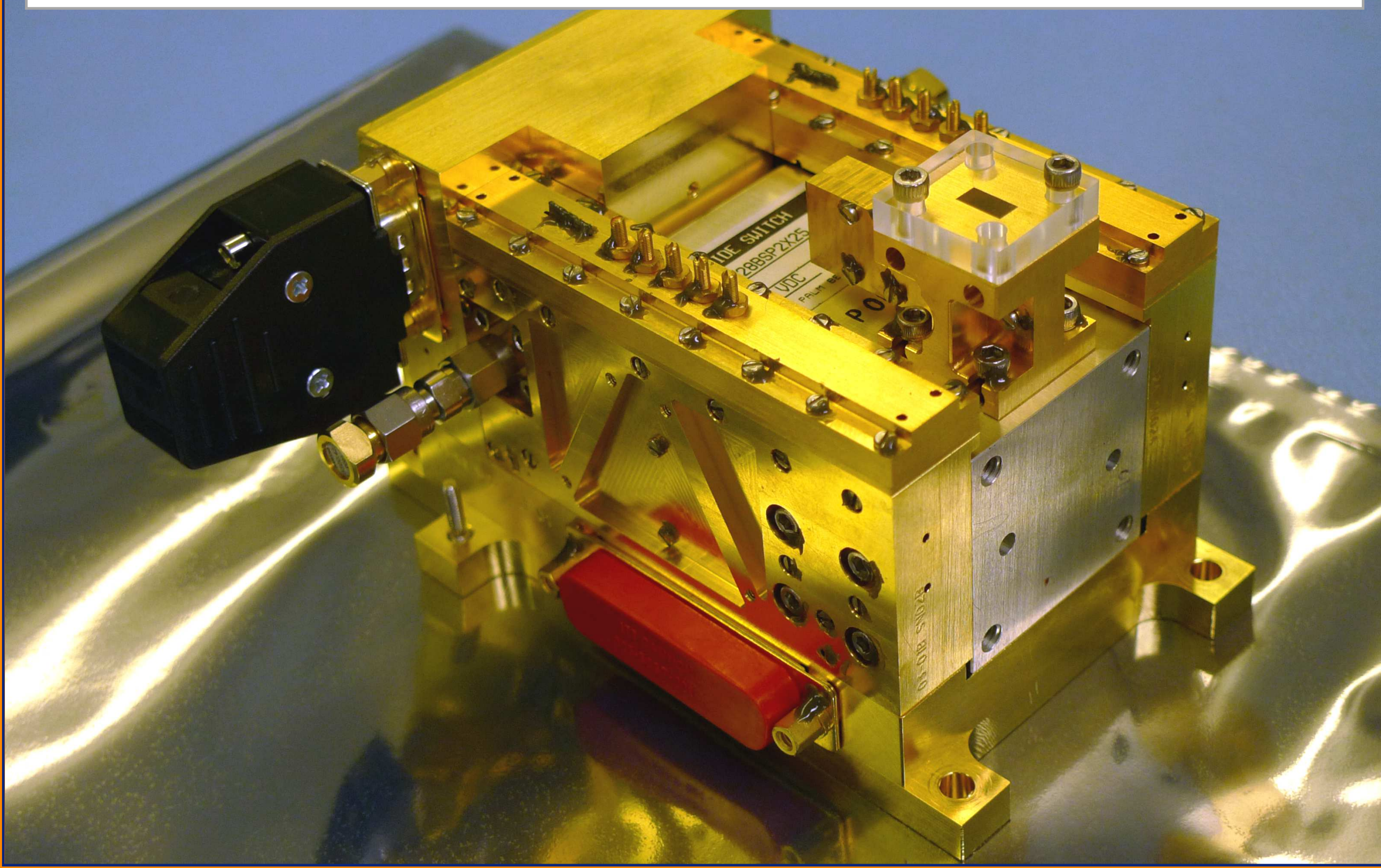
HY-2, 37 GHz dual-redun. receiver
