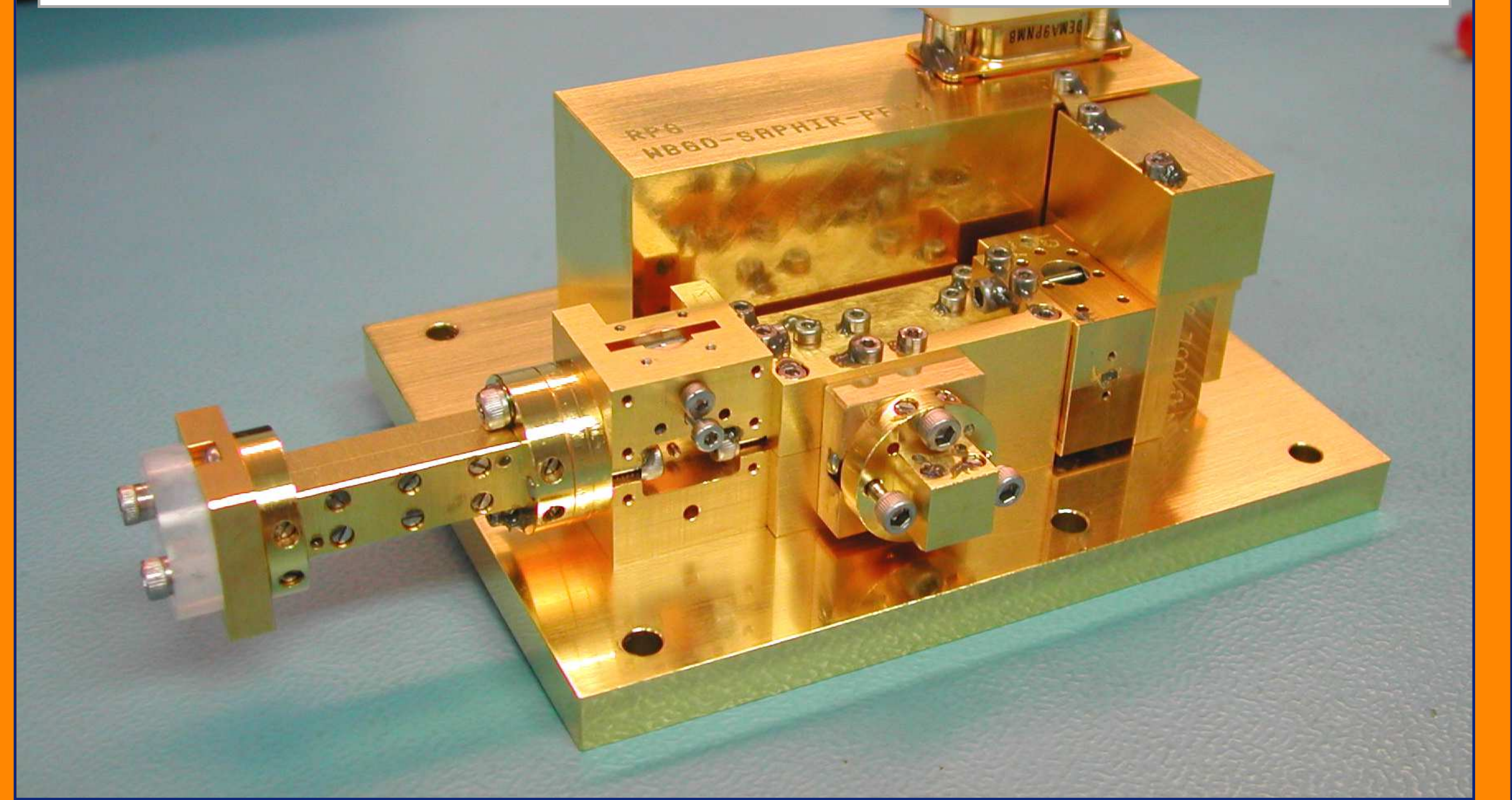
SAPHIR, Local Oscillator
