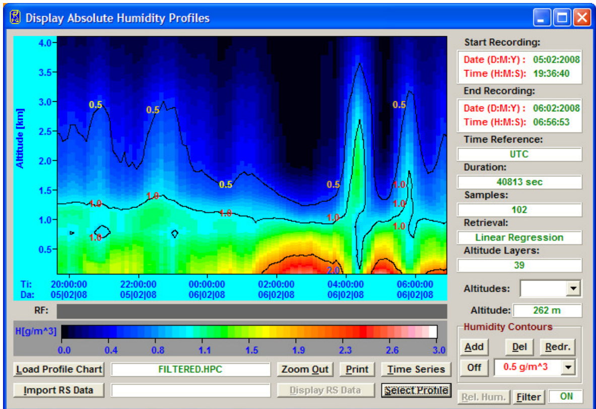
Fig.2.34: Example of humidity profile chart from Pic du Midi (French Pyrenees), courtesy of CNRS, Laboratoire d'Aerologie, Observatoire Midi-Pyrenees .
