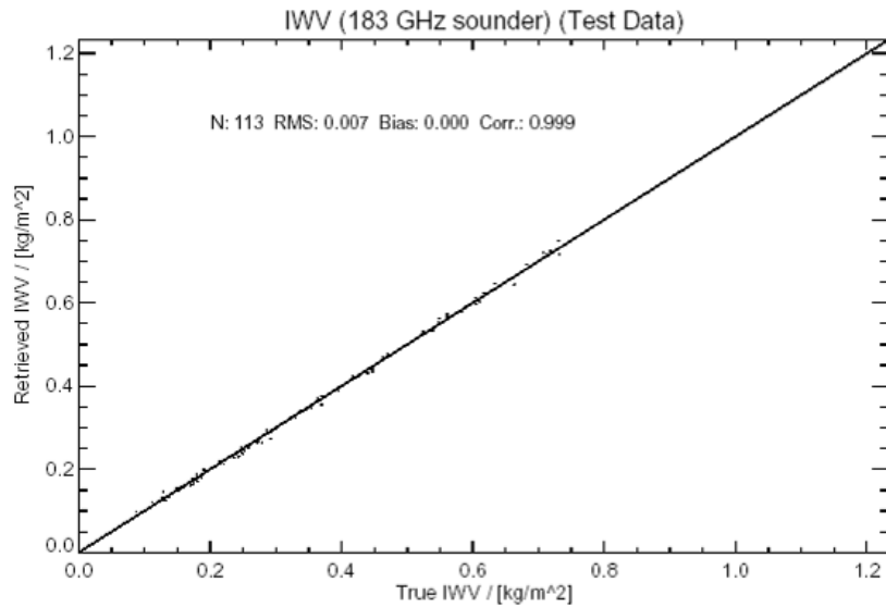
Fig.2.31: IWV scatter plot.
