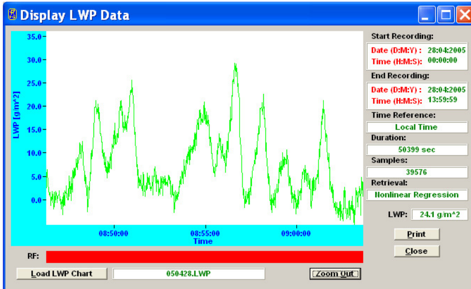
Fig.2.35: High temporal resolution (1 second sampling) LWP time series. The measurement noise is very low ( < 2 \text{ g/m}^2 RMS).
