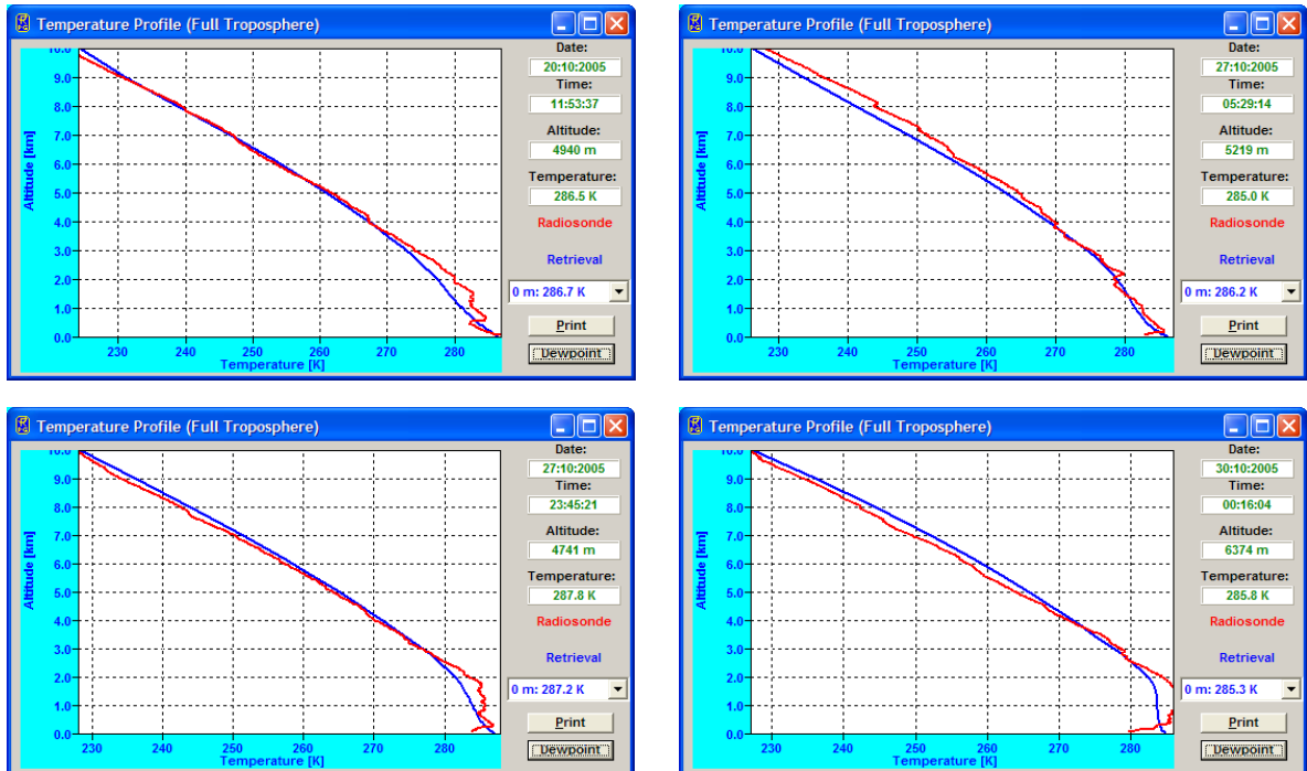
Fig.2.14a: Examples of comparisons between radio sounding (red) and HATPRO Z mode observations (blue). The boundary layer details are not always accurately resolved.
