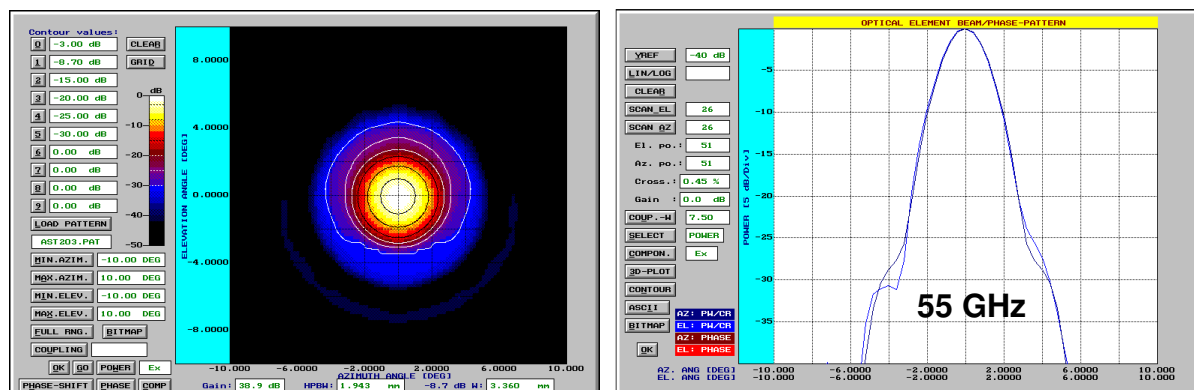
Fig.2.4: Left: 2d amplitude distributions of the parabola / corrugated feed @ 23.8 and 55 GHz. Right: H-and E-plane cuts.
