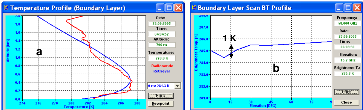
Fig.3.9: Low level temperature inversion (a) and associated brightness temperature elevation scan (b). The T_B variation in (b) is only 1 K @58 GHz for the full elevation scan ( 5^\circ to 90^\circ ).
