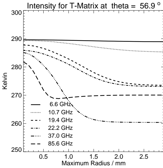
Figure 4.11: Change in brightness temperatures (using spheroid particles and a zenith angle of 56 degrees) as a function of maximum radius in the DSD integration (for details see text).
