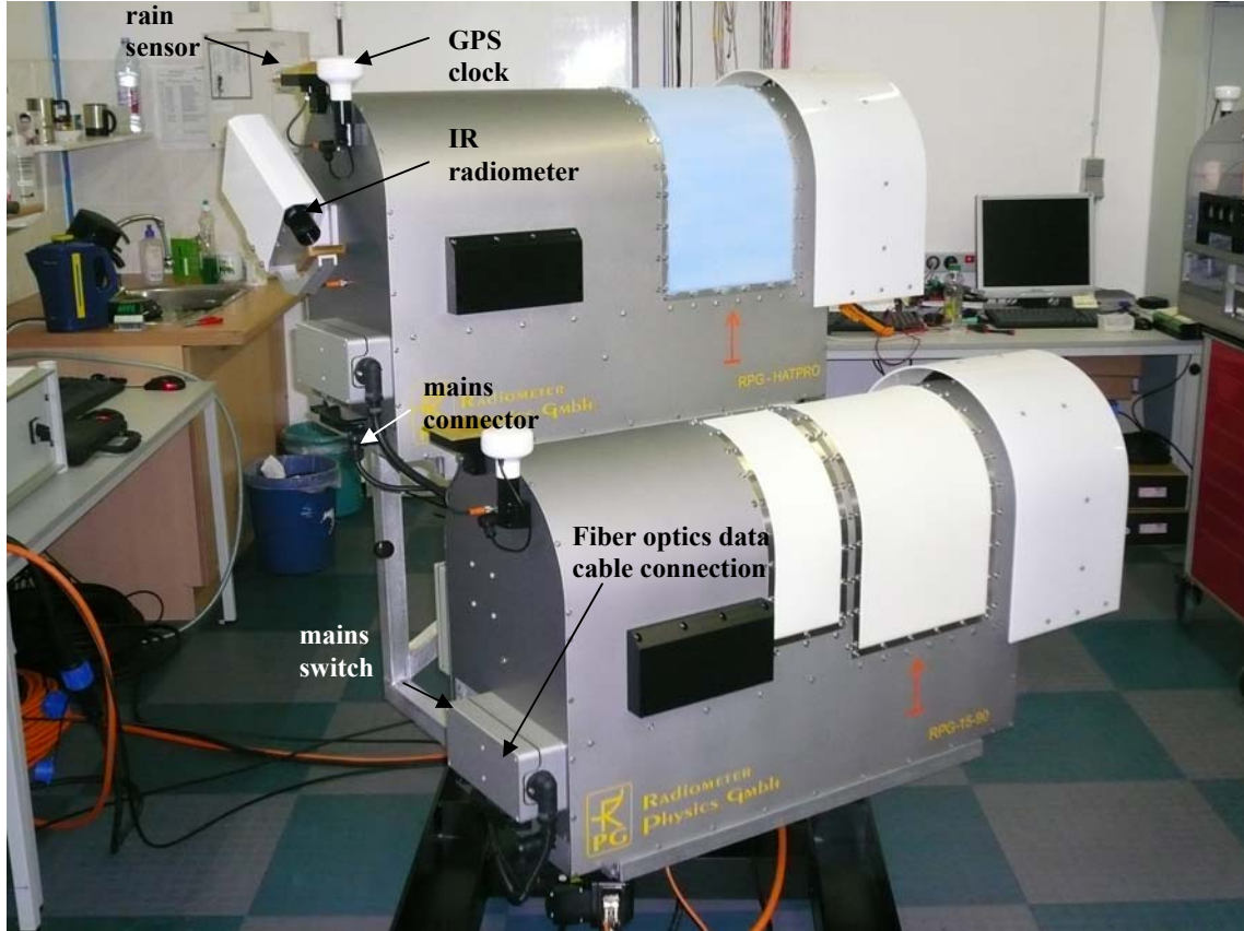
Fig.1.10: Instrument connectors and sensors (side A).
