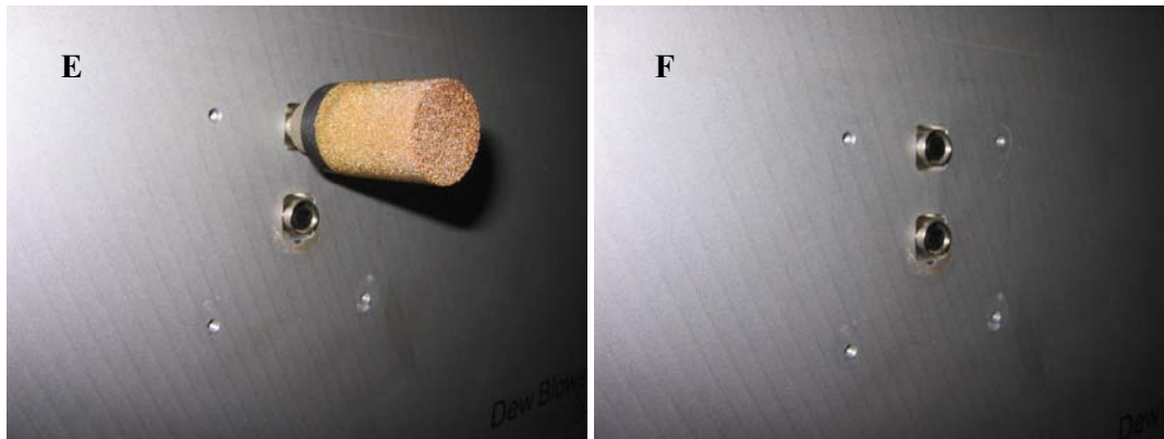
Fig.7.8A-F: Dismounting the external surface sensors: A) Sensor cage below the dew blower. B) Unscrewing the T-sensor fan. C) Unscrewing the sensor cage housing. D) The humidity sensor (with gold plated cap) and the temp. sensor can be unscrewed by hand. E) Temp. sensor removed. F) Humidity sensor removed.
