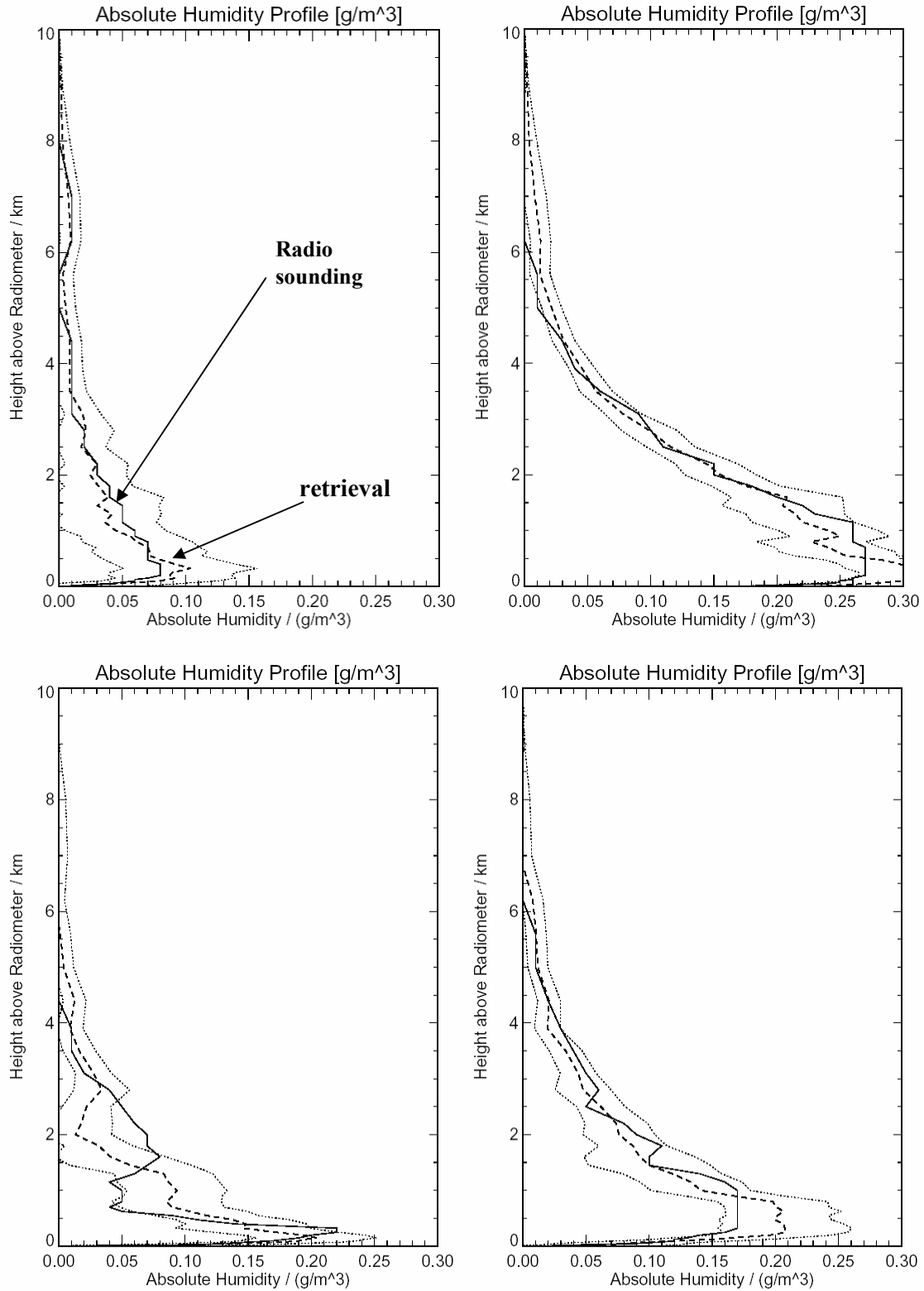
Fig.C3.1.2.3: Humidity profiling retrieval accuracy.
