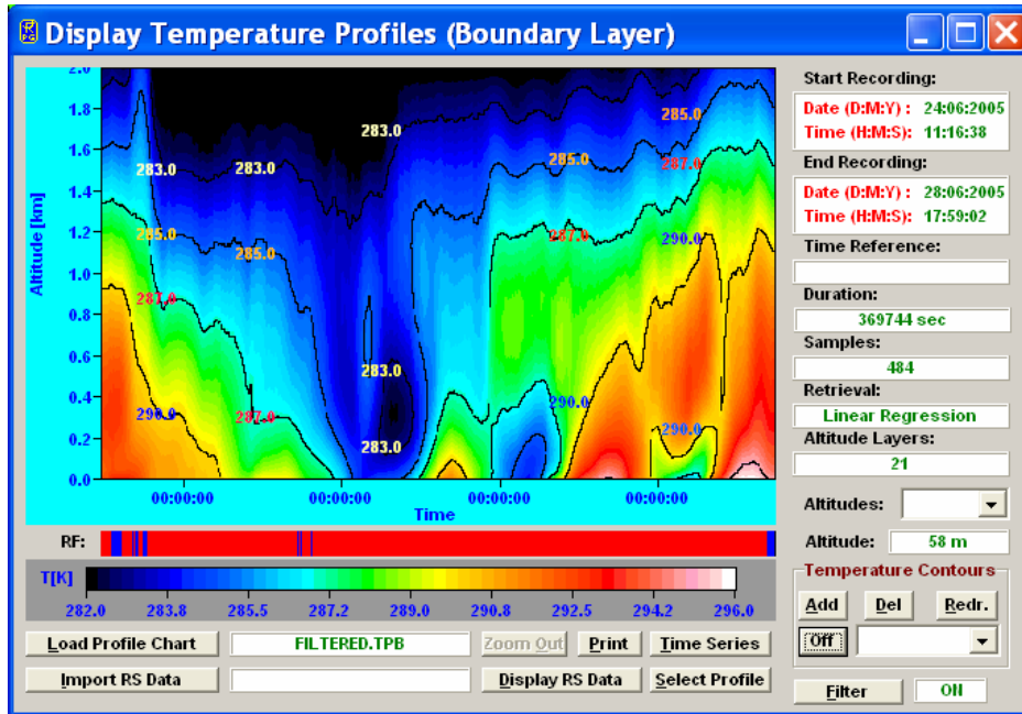
Fig.5.14a: Boundary layer temperature profile chart window.
