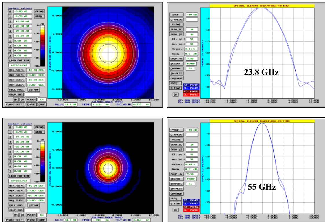
Fig.3.4: Left: 2d amplitude distributions of the paraboloid/corrugated feed @ 23.8 and 55 GHz. Right: H- and E-plane cuts.
