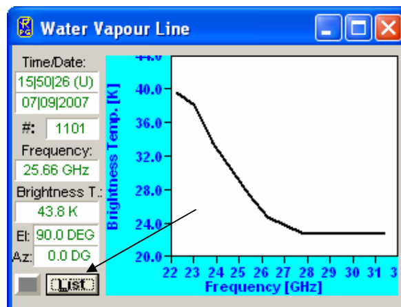
Water Vapour Line monitoring window.
