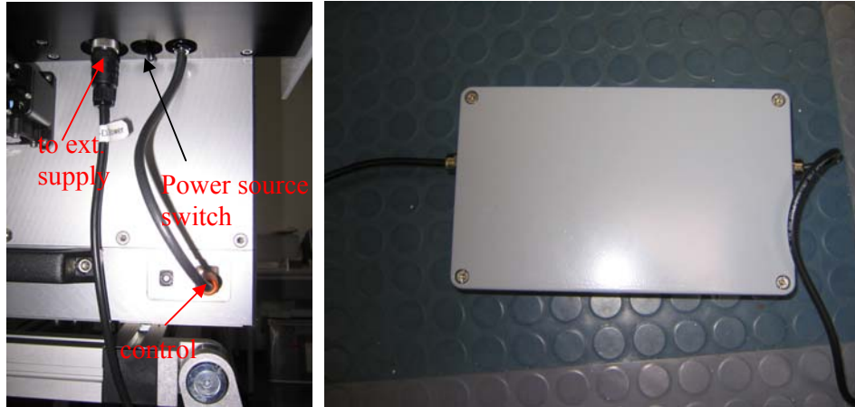
Fig.1.9: Electrical dew blower connections and external power supply.
