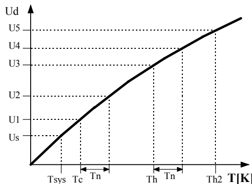
Fig.4.7: Detector response as a function of total noise temperature. T_{sys} is the system noise temperature, T_n the additionally injected noise, T_c the total noise when the radiometer is
