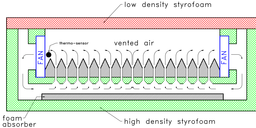
Fig.4.1: Ambient temperature target cross section.
