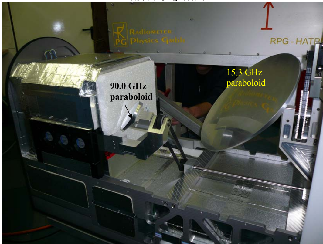
R15/90 15.3 GHz and 90 GHz direct detection receivers and their associated synchronously scanning parabola mirrors.
