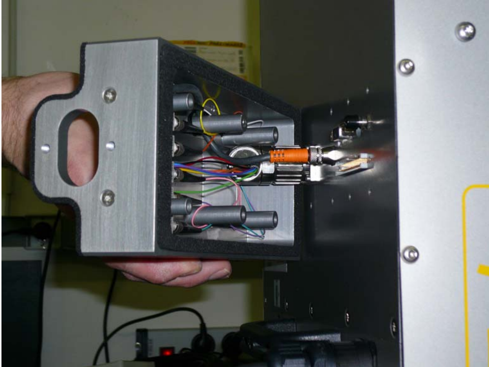
Fig.8.12a: Connect converter A to radiometer.
