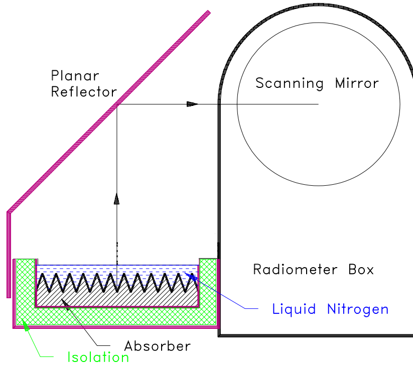
Fig.4.2: External cold load attached to the radiometer box.
