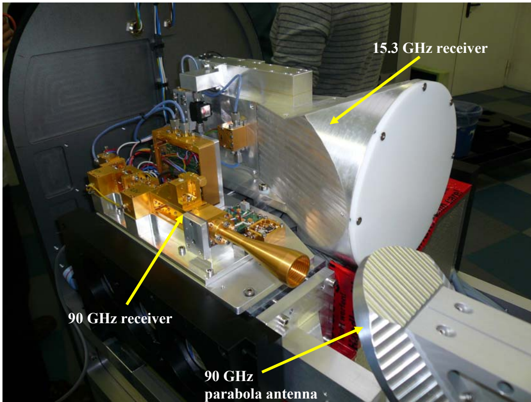
15.3 / 90 GHz receiver
