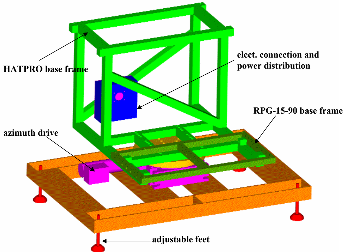
Fig.1.4: Instrument stand and azimuth table.
