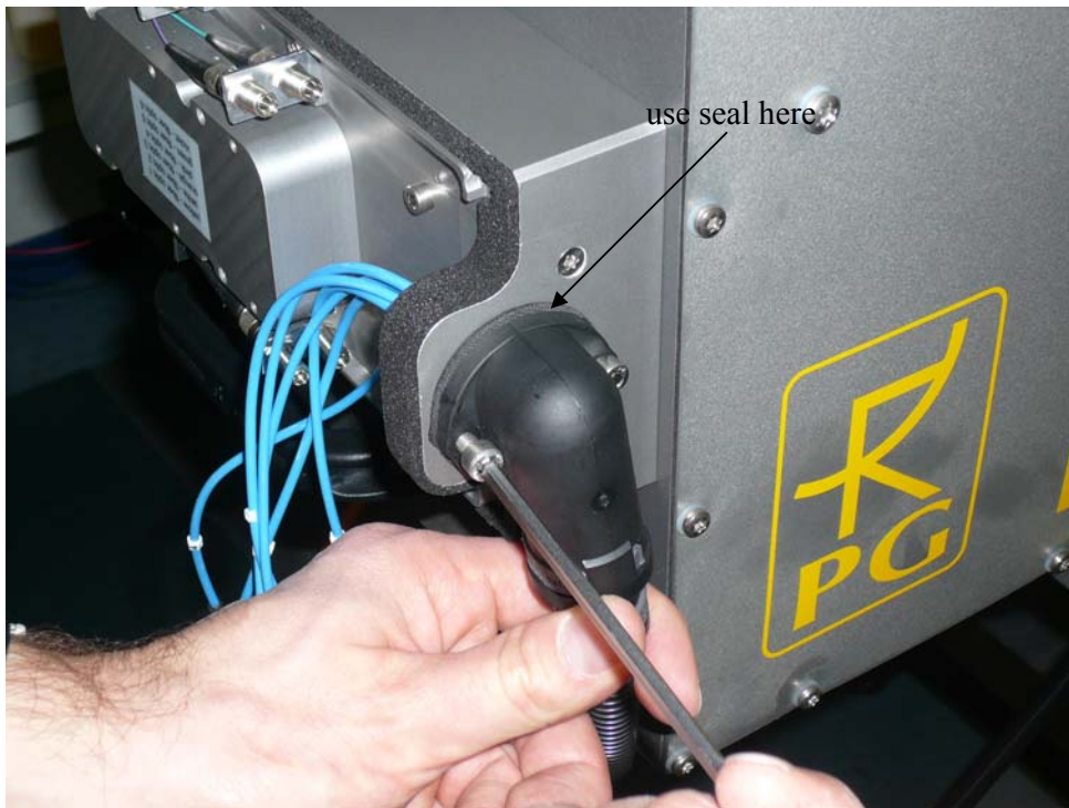
Fig.8.13b: Fiber optics cable mount.
