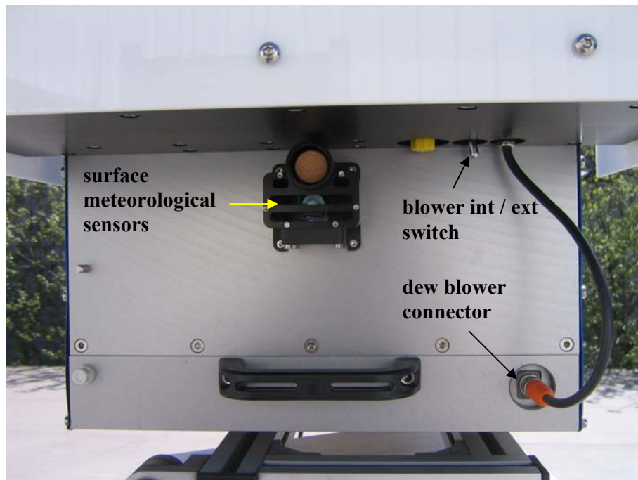
Fig.1.11: Instrument connectors and sensors on side B
