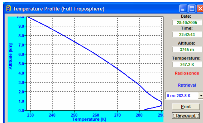
Fig.20b: Example of a composite temperature profile.
