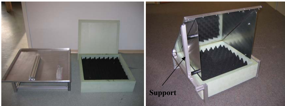
Fig.4.3: External absolute calibration target (cold load).
