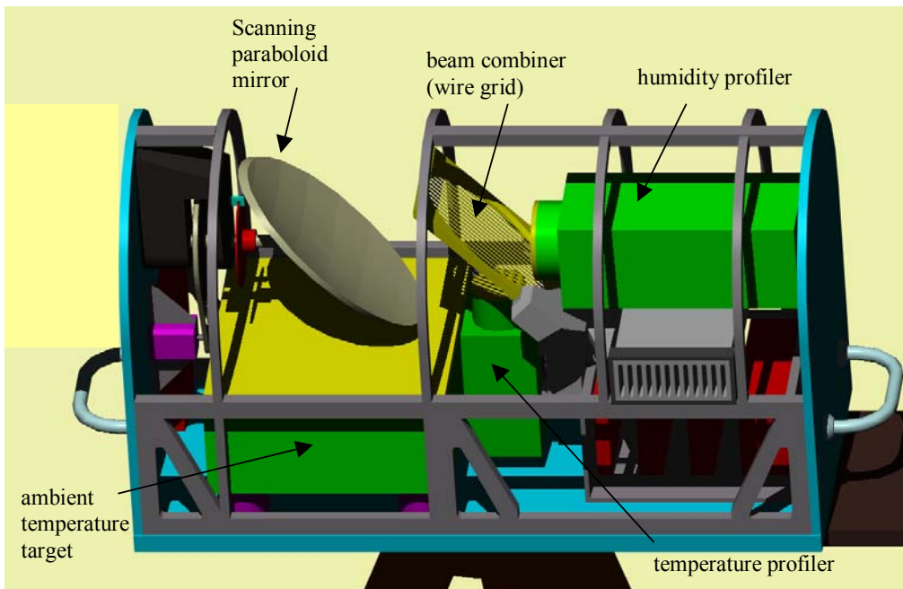
Fig. 3.1: Internal structure of the RPG-HATPRO radiometer.
