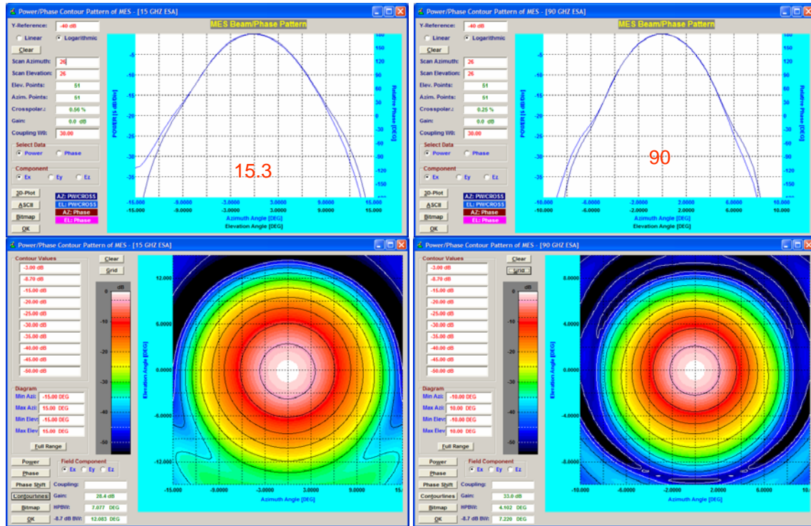
E/H plane cuts of parabola images at 15.3 and 90 GHz.
