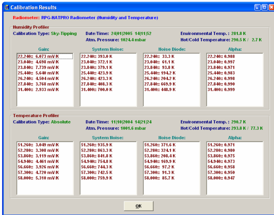
Fig.5.4: Display of absolute calibration parameters.
