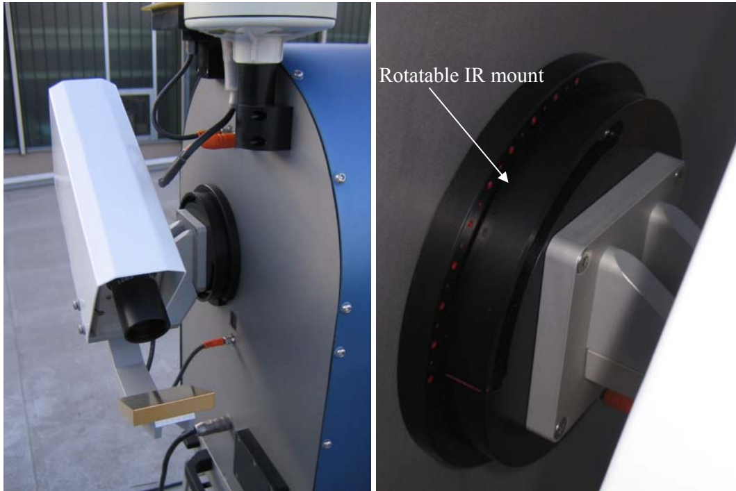
Fig.8.9: Infrared radiometer mounted to the radiometer side wall. Due to an axial mount the radiometer viewing angle can be changed between 0° and 90°.
