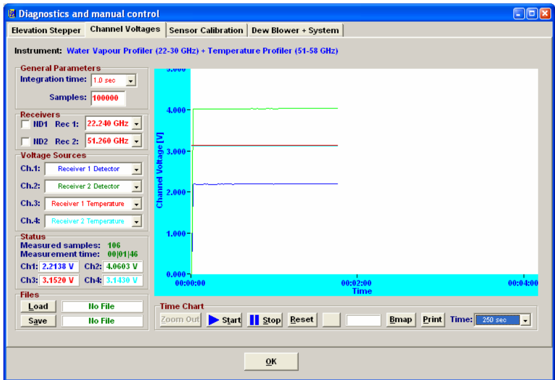
Fig.5.22: Channel voltages tab sheet.
