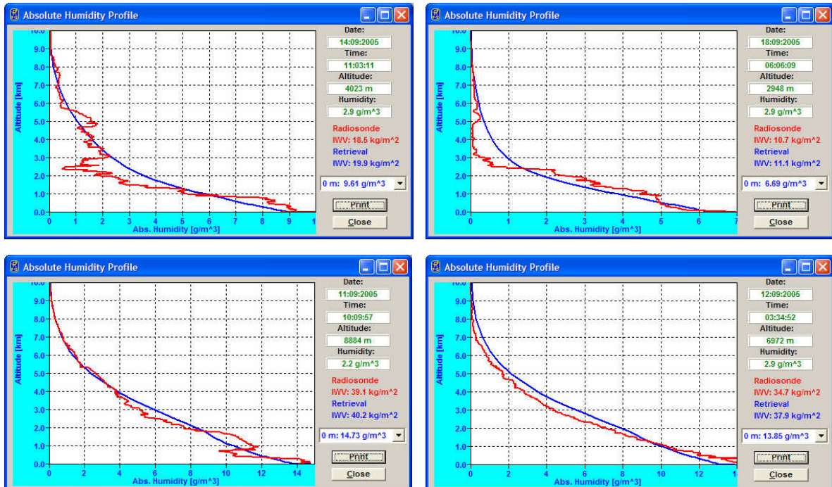
Fig.2.24: Absolute humidity profiles compared to radio soundings (red). Statistical analysis leads to RMS errors of 1 g/m 3 .
