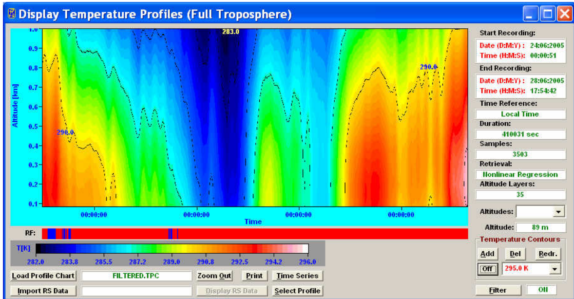
Fig.2.3a: Zenith observation mode. In the lower 500 m layer the vertical structure is hardly resolved.
