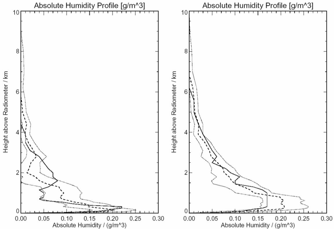
Fig.2.32: Humidity profiling retrieval accuracy.
