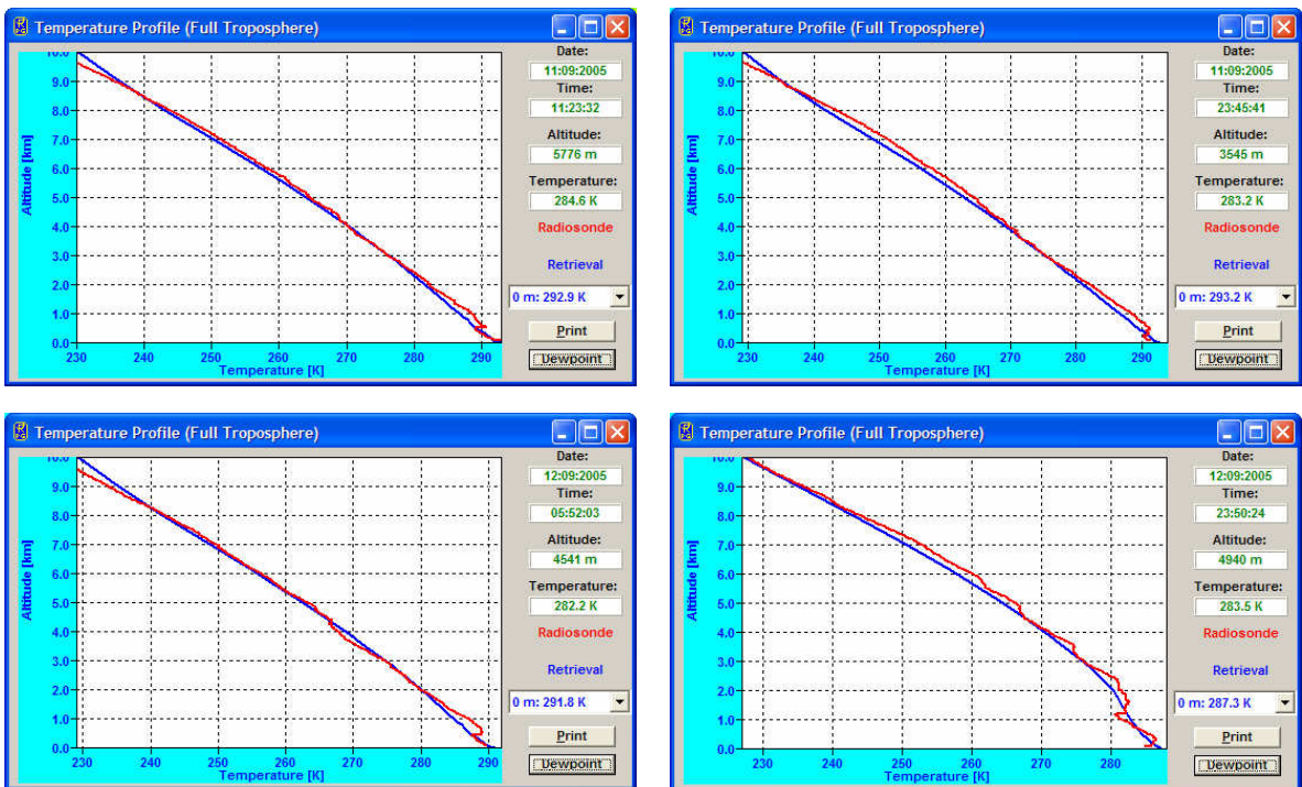
Fig.2.14b: The Z mode tends to smear out (average) the details of the boundary layer.
