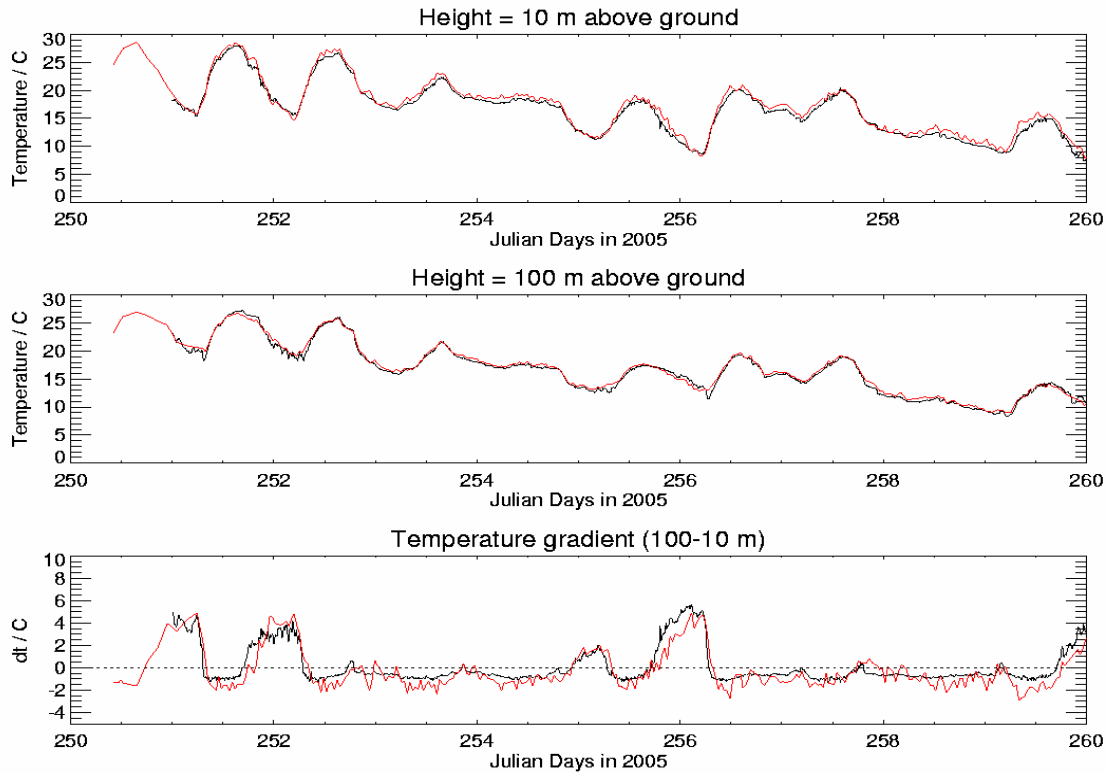
Fig.2.8a: Comparison of time series of tower temp. sensor (black) and HATPRO measurement (red) at 10 m and 100 m. Below is shown the gradient (difference) indicating that all low level inversions were captured by the instrument.
