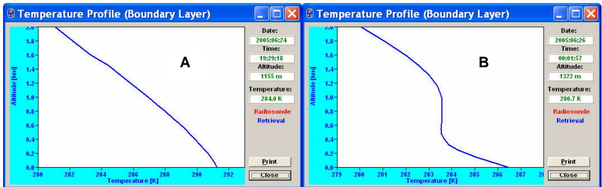
Fig.2.4: Boundary layer scan temperature profile map of the lowest 2000 m layer. Examples of different scans are given below. The time of the diagram is measured in UTC. 00:00:00 corresponds to midnight.
