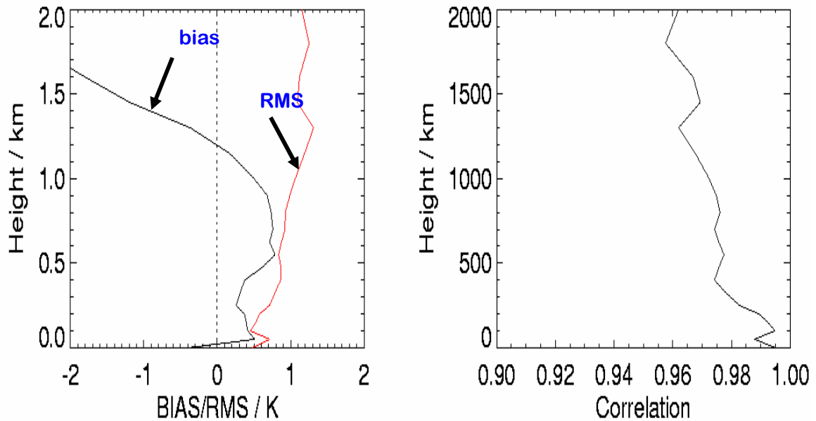
Fig.2.9: RMS and bias of the BLM temperature observations. Due to the 4 km distance between radio sounding and radiometer the details of the boundary layer are not necessarily the same. The BLM data is most accurate for altitudes < 1200 m.
