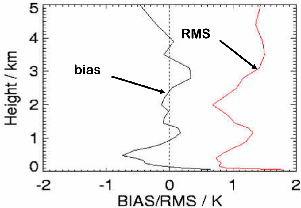
Fig.2.10: RMS and bias of the ZM temperature observations..
