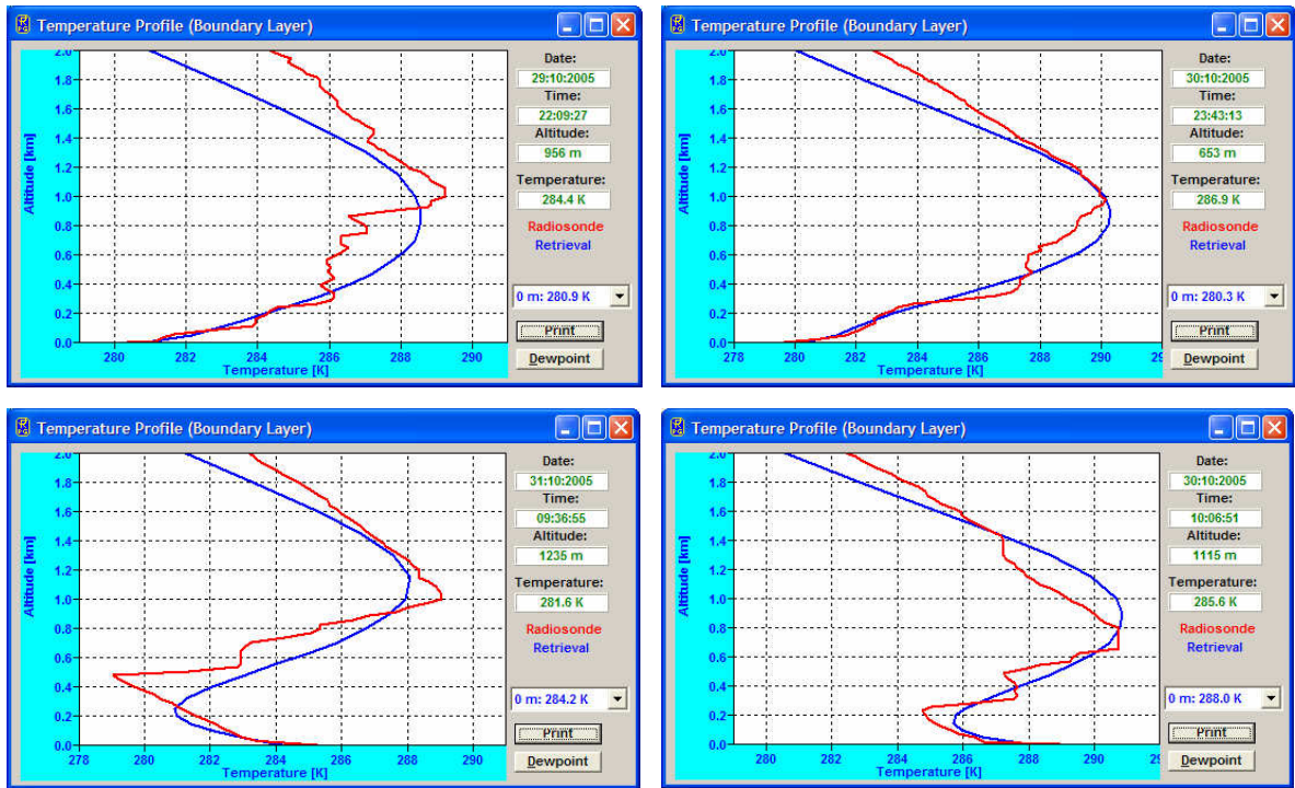
Fig.2.13: Inversion comparisons between radio sounding (red) and HATPRO BL mode observations (blue) for the four cases in fig.10 indicated by the black lines.
