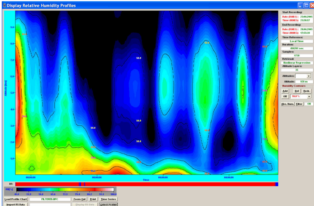
Fig.2.19: Relative humidity map for the full troposphere (up to 10 km) computed from absolute humidity profiles and temperature profiles both measured in zenith mode.
