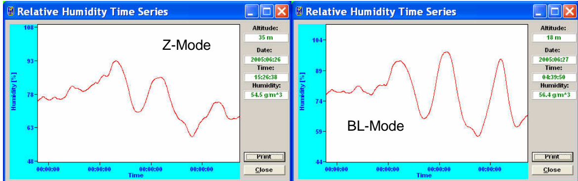
Fig.2.23: Relative humidity time series at low altitude measured in Z-mode and BL-mode. The BL-mode humidity maxima over night between 22:00 and 7:00 (when inversions are generated) are more pronounced than in Z-mode.
