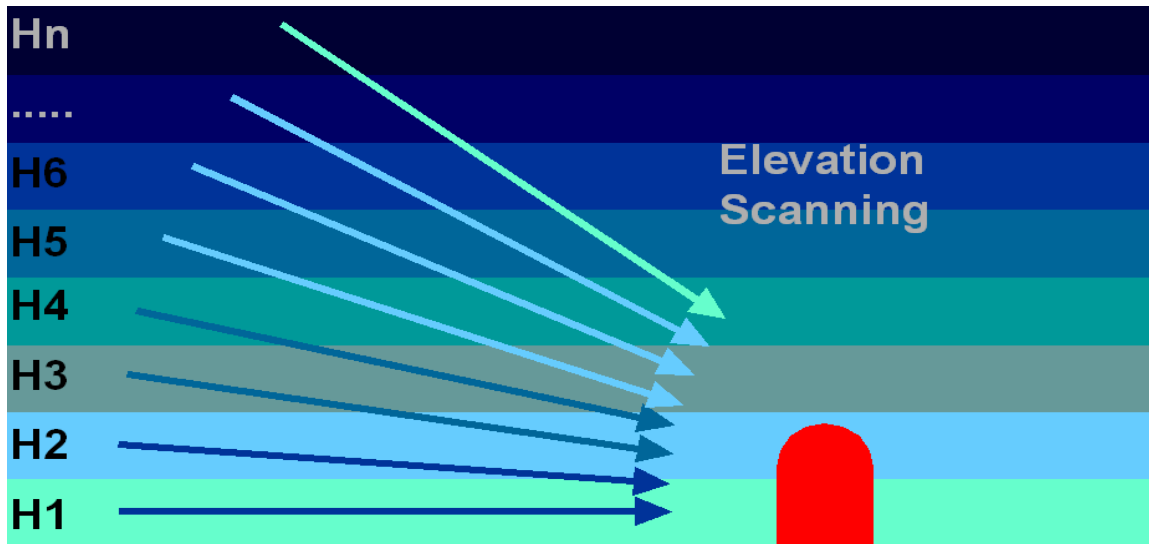
Fig.2.2: Boundary layer scanning mode with different elevation angles.
