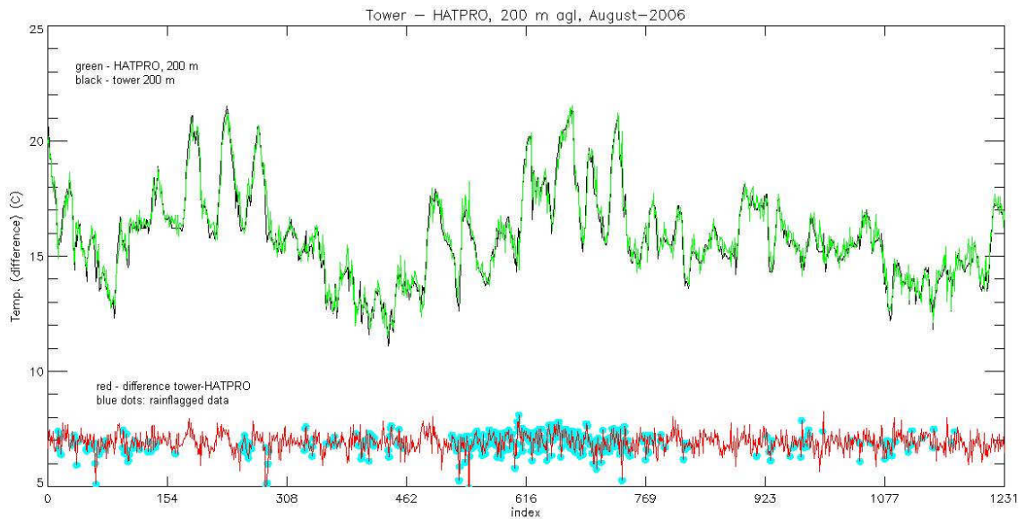
Fig.2.11: Comparison of retrieved HATPRO temperature at 200 m (green) with 200 m temperature sensor reading of met. tower (black) in Cabauw (KNMI) in August 2006. Total number of samples: 1232, no-rain: 836 samples (RMS: 0.36 K, bias: -0.04 K); 396 rain samples (RMS: 0.45 K, bias: -0.13 K). Rain samples are indicates as blue dots, rain rates are between 1 mm/h (drizzle) and 25 mm/h. BLM data remains accurate.
