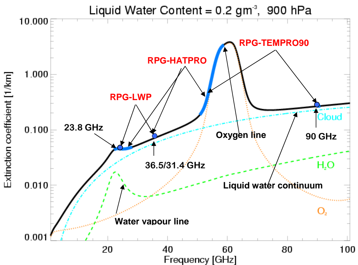
Fig.2.1: Frequency sets observed in zenith observation mode by various RPG instruments.
