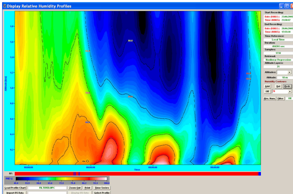
Fig.2.22: Relative humidity map for boundary layer (up to 2 km) computed from absolute humidity profiles and temperature profiles measured in boundary layer mode. A comparison with Fig.13 clearly shows that more details are resolved in the <500 m range. The relative humidity is modulated by the temperature inversions.
