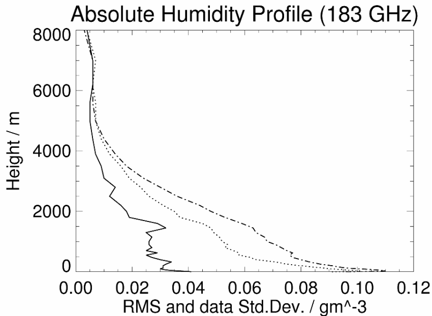
Fig.2.30: Retrieval accuracy for humidity profiling with the 22 GHz and 183 GHz water vapour line.
