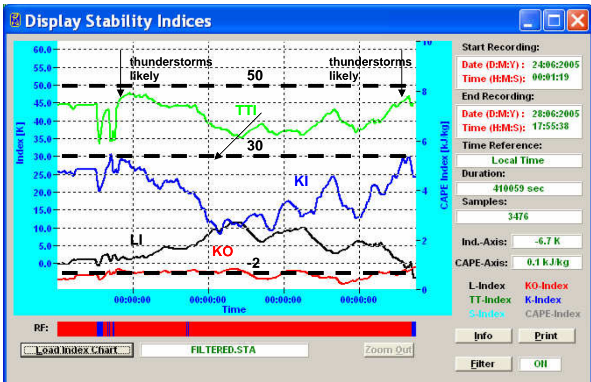
Fig.2.38: When TTI, KI and LI are approaching their critical limits, thunderstorms are likely to occur. This can be seen from the rain flag bar (blue indicates 'rain', red means 'no rain').
