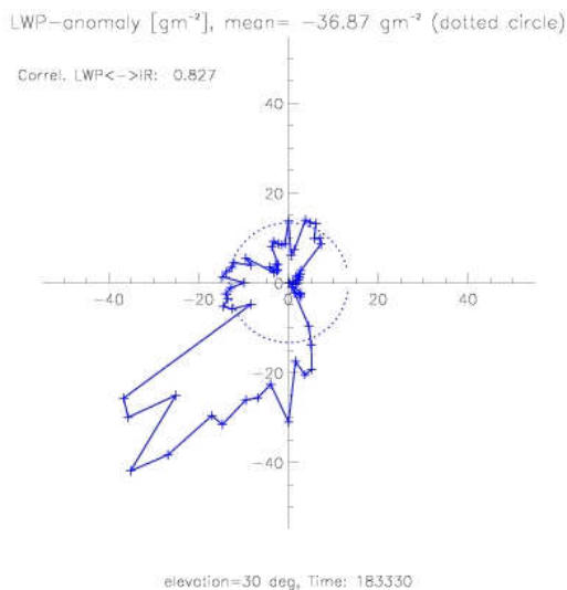
Fig.2.42: Under cloudy conditions, the IR radiometer signal is partially saturated while the microwave IWV is still reflecting the water vapour distribution. The IR gets saturated where the LWP level indicates clouds. Courtesy of S. Kneifel, Univ. of Cologne and LMU Munich.
