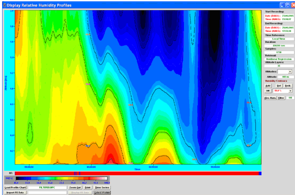
Fig.2.21: The lowest 2000 m layer map of Fig.2.11 computed from absolute humidity profiles and temperature profiles both measured in zenith mode.
