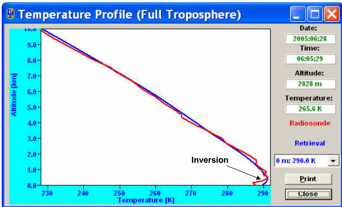
Fig.2.5: Full troposphere (zenith) scan. Inversion below 1 km is not well resolved (about 1 K)
