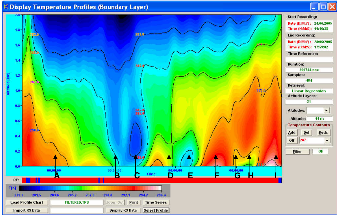
Fig.2.4: Boundary layer scan temperature profile map of the lowest 2000 m layer. Examples of different scans are given below. The time of the diagram is measured in UTC. 00:00:00 corresponds to midnight.
