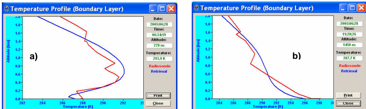
Fig2.6: a) Radiosonde (red) and boundary layer scan (blue) profiles at the same time as above. A strong ground inversion of 4K is resolved. b): Boundary layer scan around 12:00 UTC. The inversion has disappeared.
