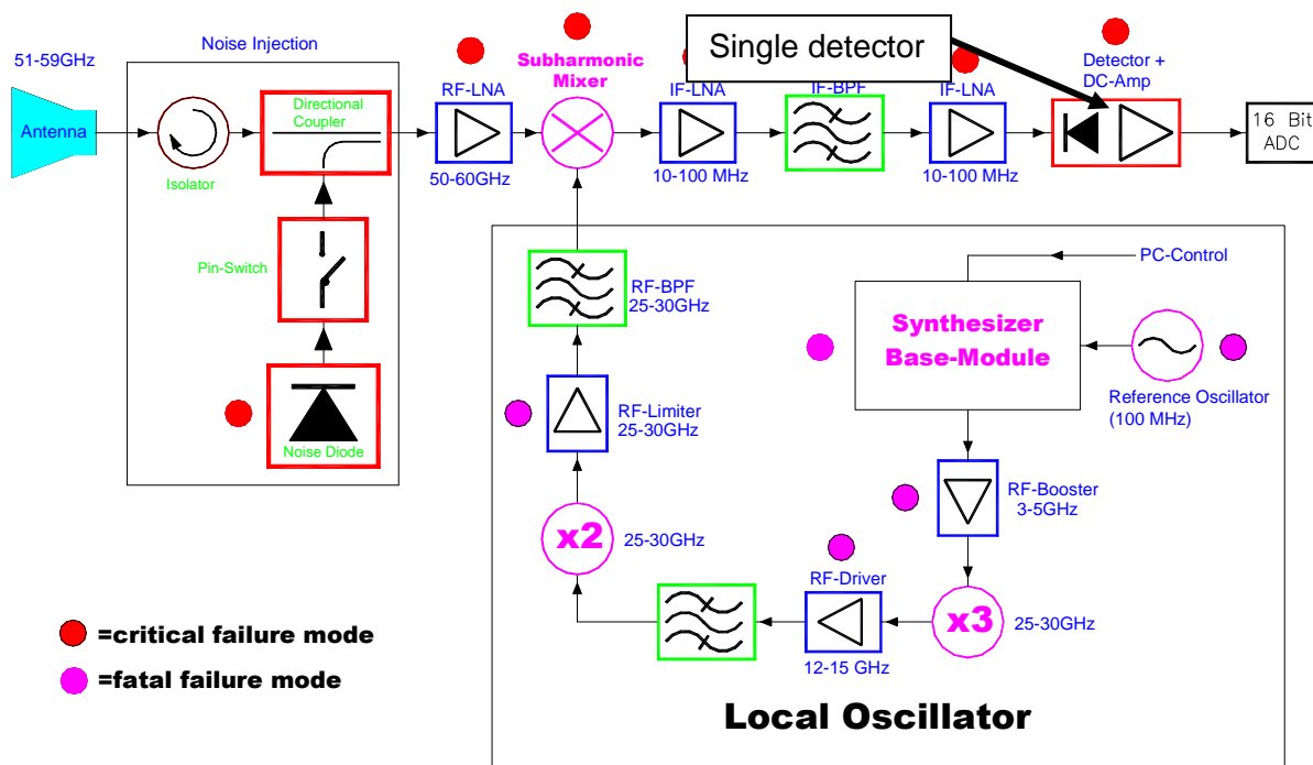
Fig.3.3: Single channel spectrum analyzer with sequential frequency scanning.
