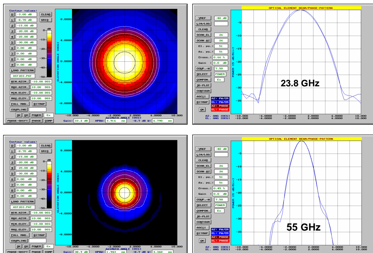
Fig.2.4: Left: 2d amplitude distributions of the parabola / corrugated feed @ 23.8 and 55 GHz. Right: H- and E-plane cuts.
