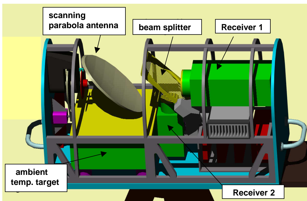
Fig. 2.1: Schematic internal structure of un-polarized RPG radiometers.
