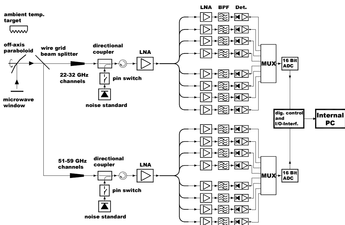
Fig.2.2a: Example of RPG-HATPRO schematic receiver layout. Both radiometers are direct detection systems without the need for local oscillators and mixers.
