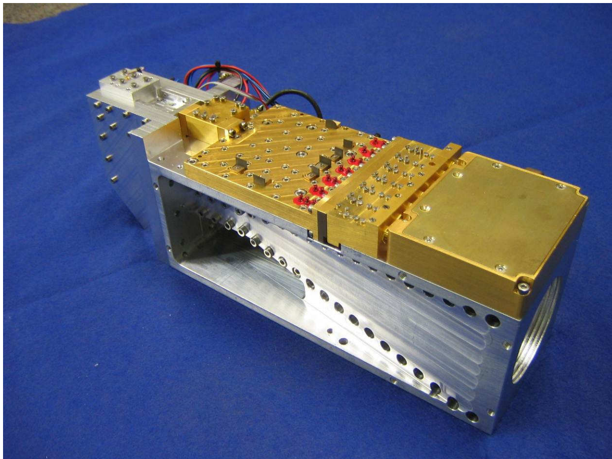
Fig.2.3: Temperature profiling direct detection filter bank receiver mounted to the 50-60 GHz corrugated feedhorn. Receiver size: 72 x 200 x 15 mm 3 .
