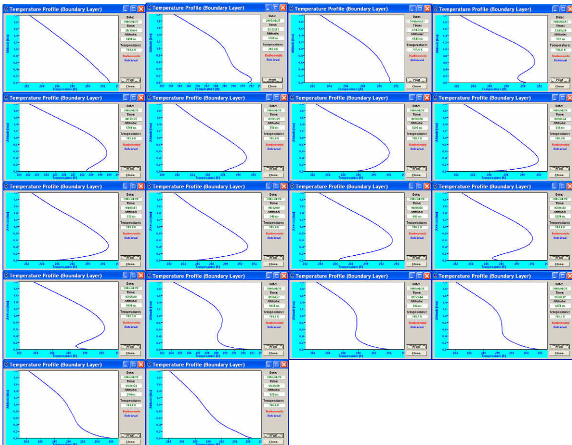
Fig.3.10: Development and decay of temperature inversions.
