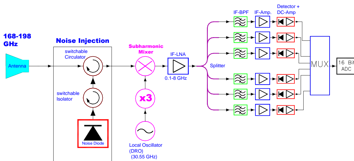
Fig.2.2b: Example of RPG-LHATPRO 183 GHz water vapour radiometer schematic receiver layout. The system is equipped with a new 160-200 GHz calibration noise source, allowing for a full internal auto-calibration without the need for heated or cooled calibration targets.
