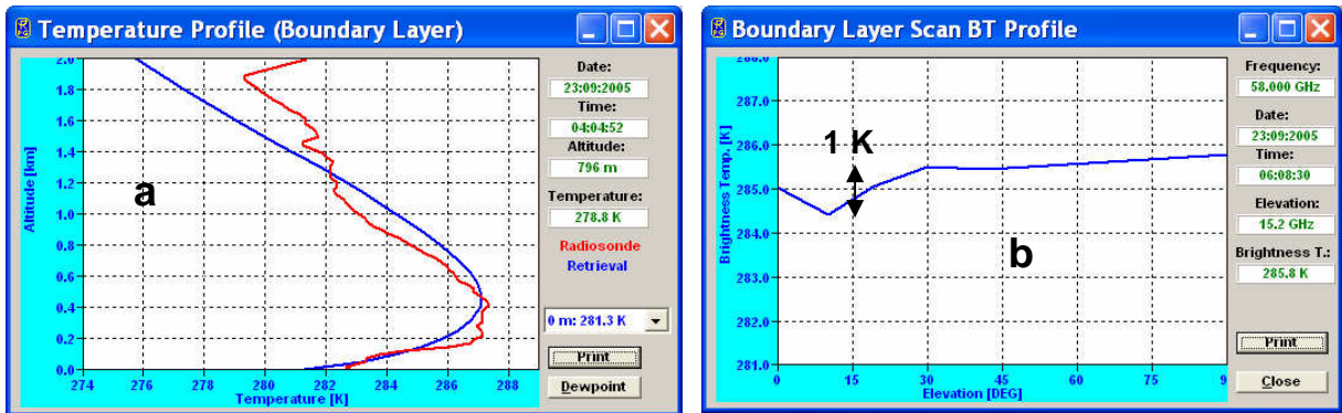
Fig.3.9: Low level temperature inversion (a) and associated brightness temperature elevation scan (b). The T_B variation in (b) is only 1 K @58 GHz for the full elevation scan (5° to 90°).
