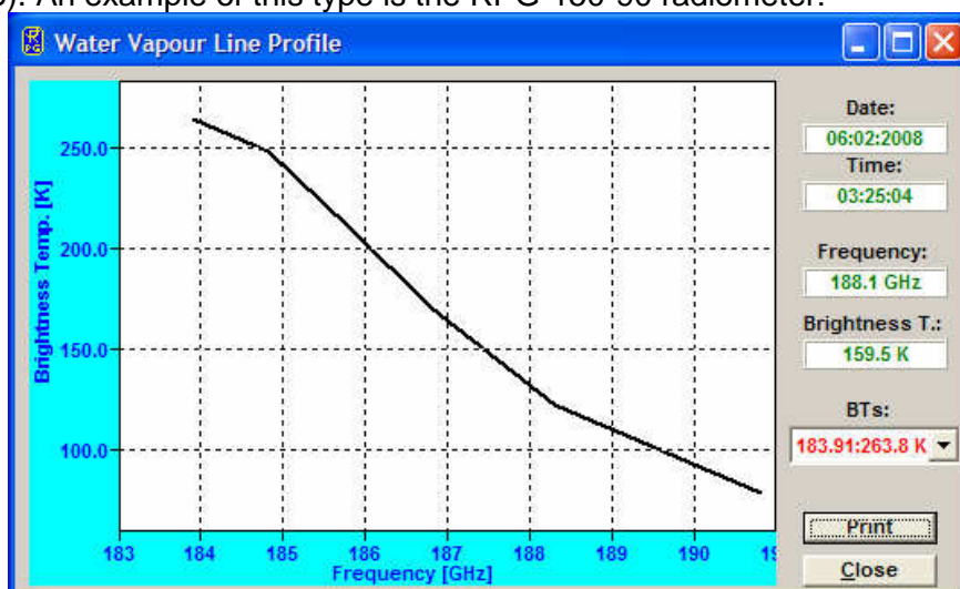
Fig.2.2d: RPG-LHATPRO 183 GHz water vapour line observed on Pic du Midi (2977 m asl) in the French Pyrenees (courtesy of CNRS, Laboratoire d'Aerologie, Observatoire Midi-Pyrenees).
