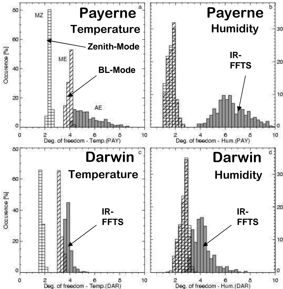
Fig.3.6: Comparison of degrees of freedom for different scanning modes (Boundary Layer scanning BL-Mode and Zenith Observation Mode) and data from an infrared FFTS spectrometer (to be ignored in this context).
