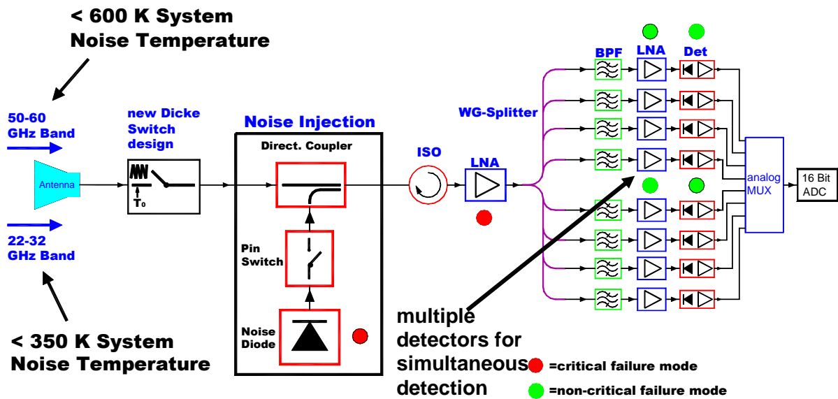
Fig.3.2: Direct detection filterbank receiver layout with failure modes.
