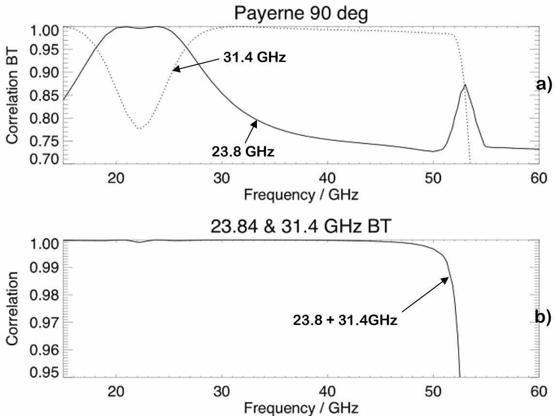
Fig.3.5: a): Correlation between the 23.8 / 31.4 GHz BT with the spectrum between 15 GHz and 60 GHz, b): Correlation between frequency pair 23.8 / 31.4 GHz and 15-60 GHz spectrum.
