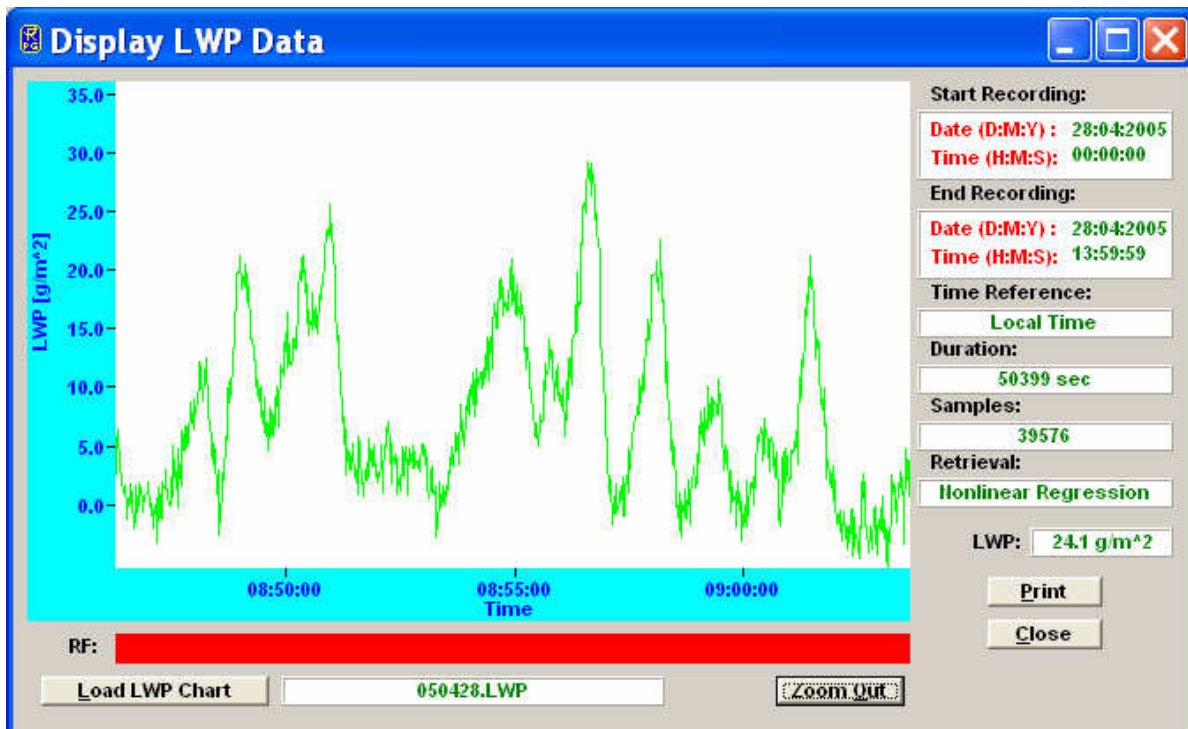
Fig.3.12: High temporal sampling required for LWP measurements (e.g. cloud modelling).
