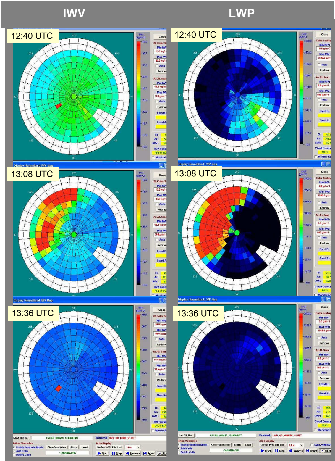
Fig.3.11: Sky volume scans of IWV and LWP with 340 points, showing an inhomogeneous humidity field (frontal passage)
