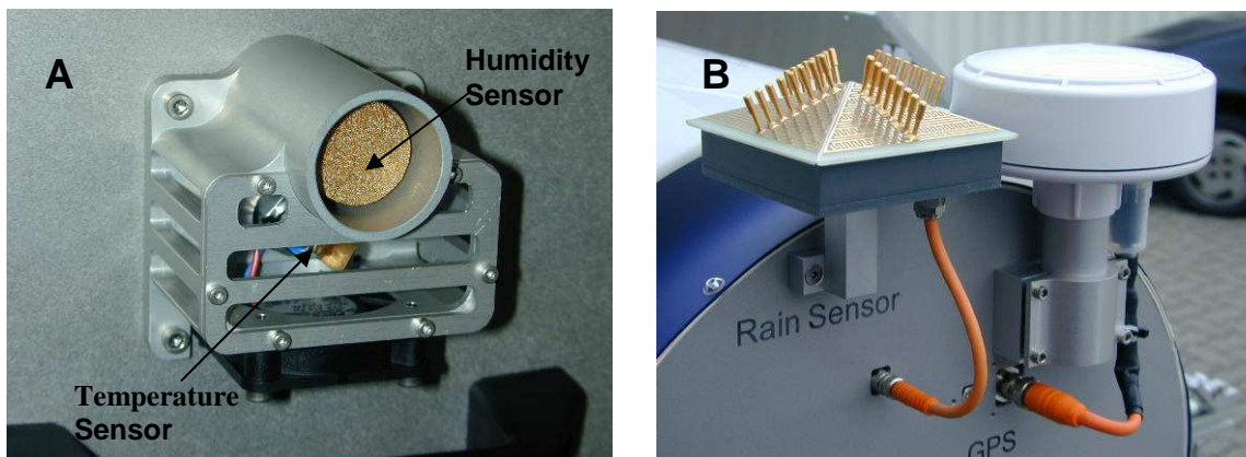
Fig.2.5: External Sensors: A) humidity and temperature sensors, B) rain sensor and GPS receiver.
