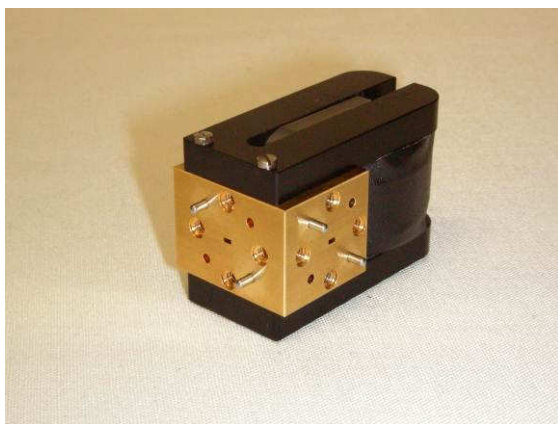
Fig.2.2f: Left: Narrow band 90 GHz y-junction Dicke Switch (transmission loss 0.6 dB, right: Full W-band Faraday Dicke Switch (transmission loss 1.0 dB).
