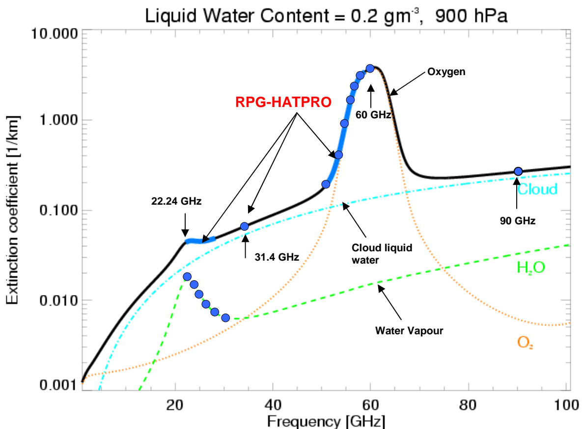
Fig.3.1: Spectral features used for microwave atmospheric profiling
