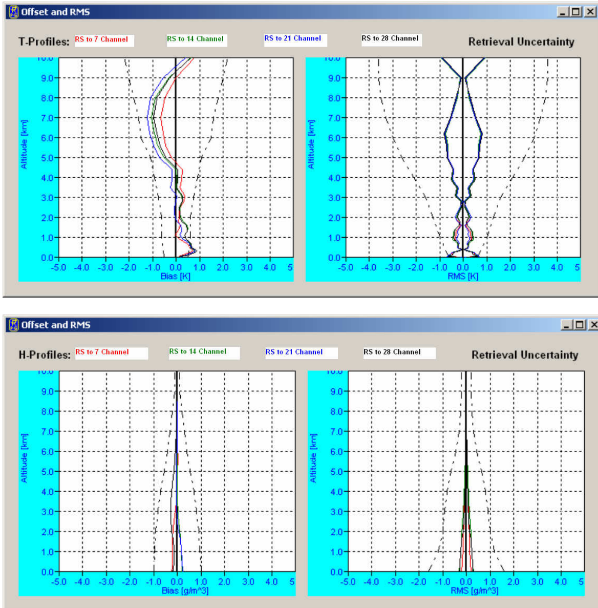
Fig.3.7: Comparison of temperature (top) and humidity (bottom) profile accuracy for 4 different radiometers operating on 7, 14, 21 and 28 different channels per line.
