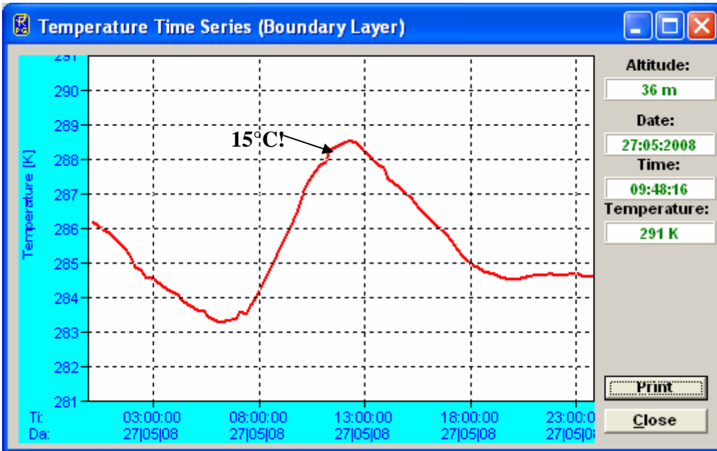
Temperature time series measured by the BL profiling method close to the ground
