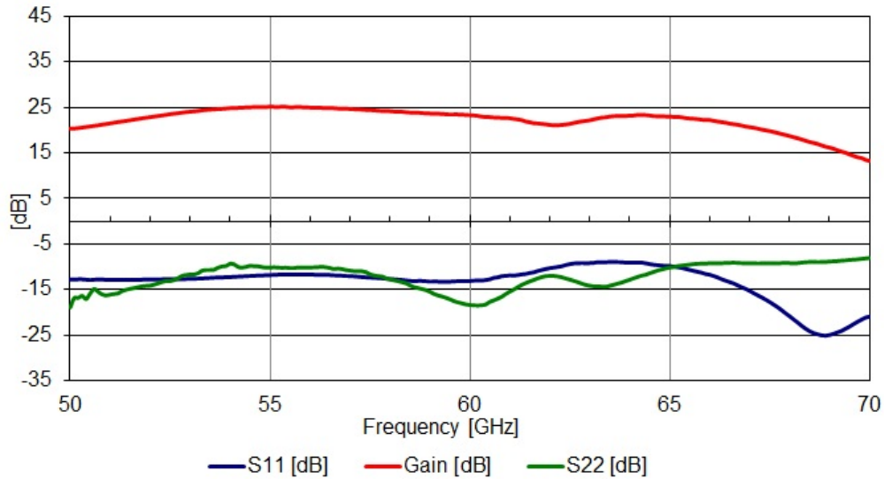
V-MPA 50-70 24 16 - Gain and Return Loss Performance
