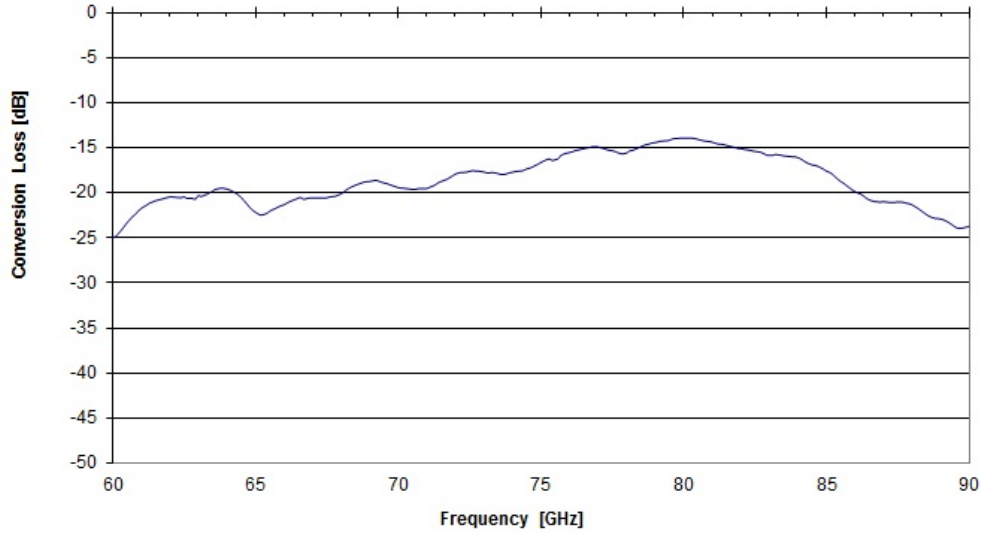
Conversion Loss FS-Z90
