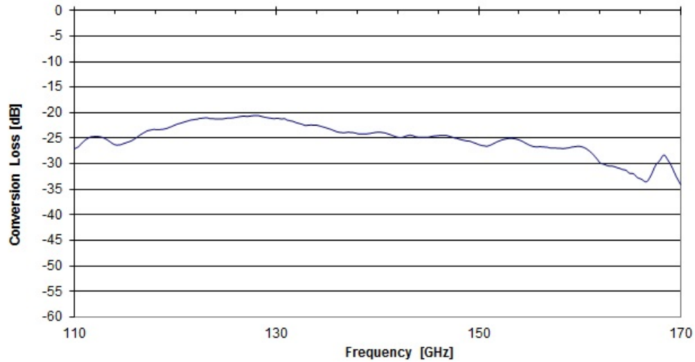
HM-170 - Conversion Loss
