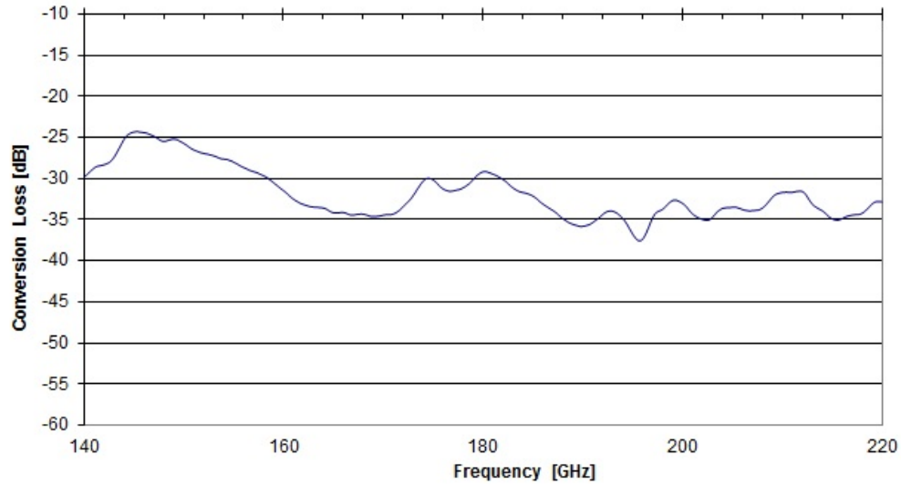
HM-220 - Conversion Loss
