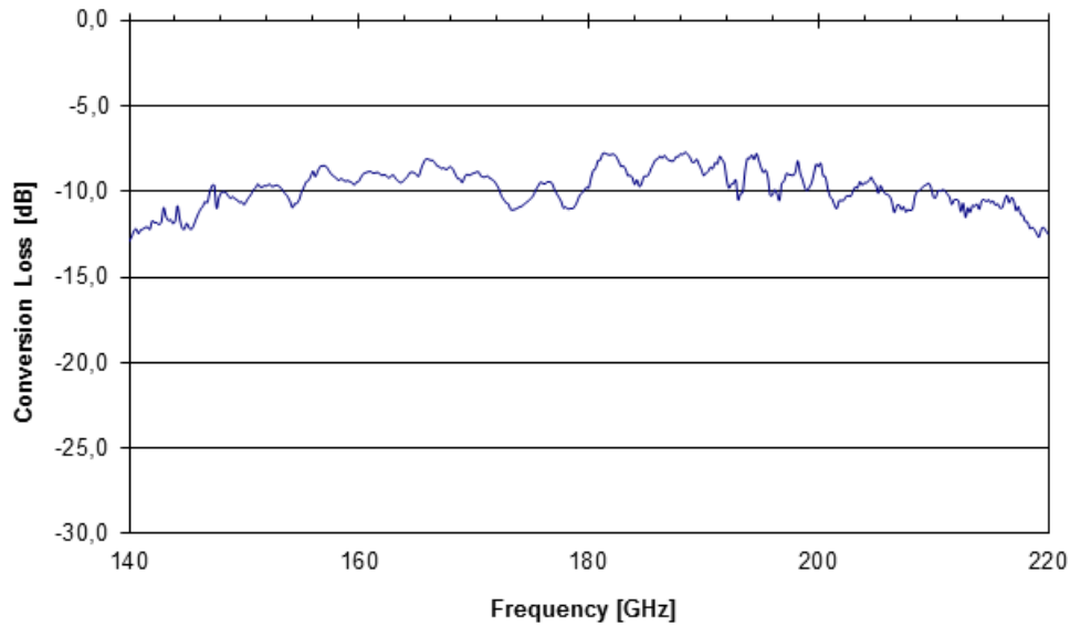
SHM-220 Conversion Loss
