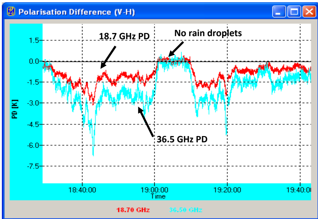
Fig. 4 Polarization Difference for rain and cloud mixtures
