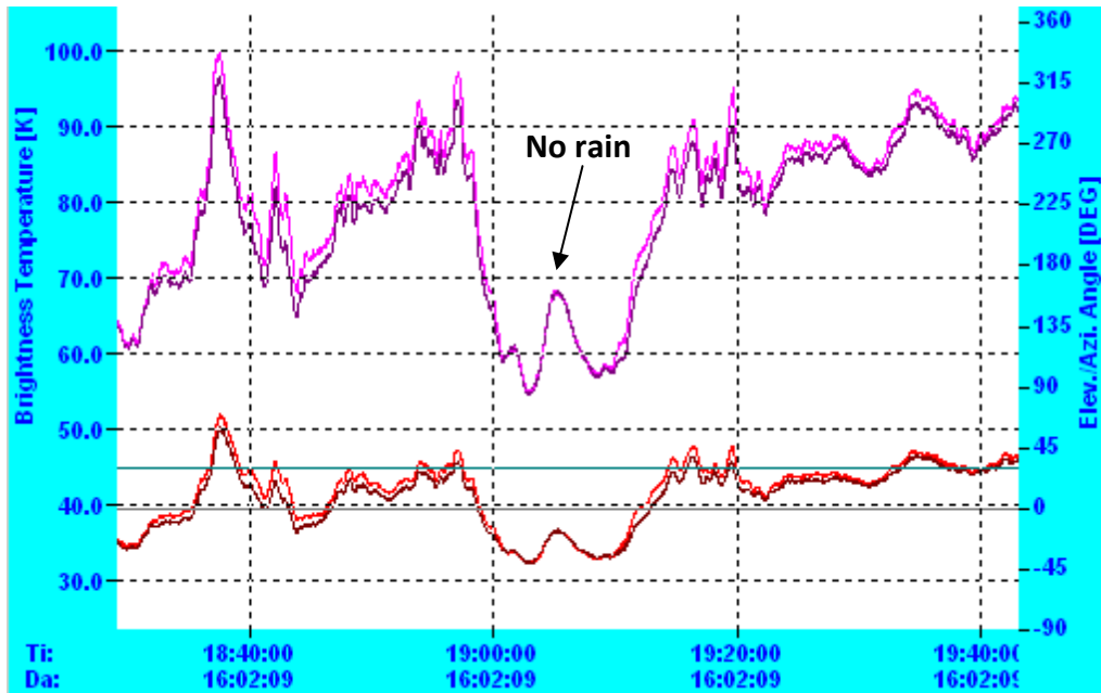
Fig. 3 Brightness Temperature
